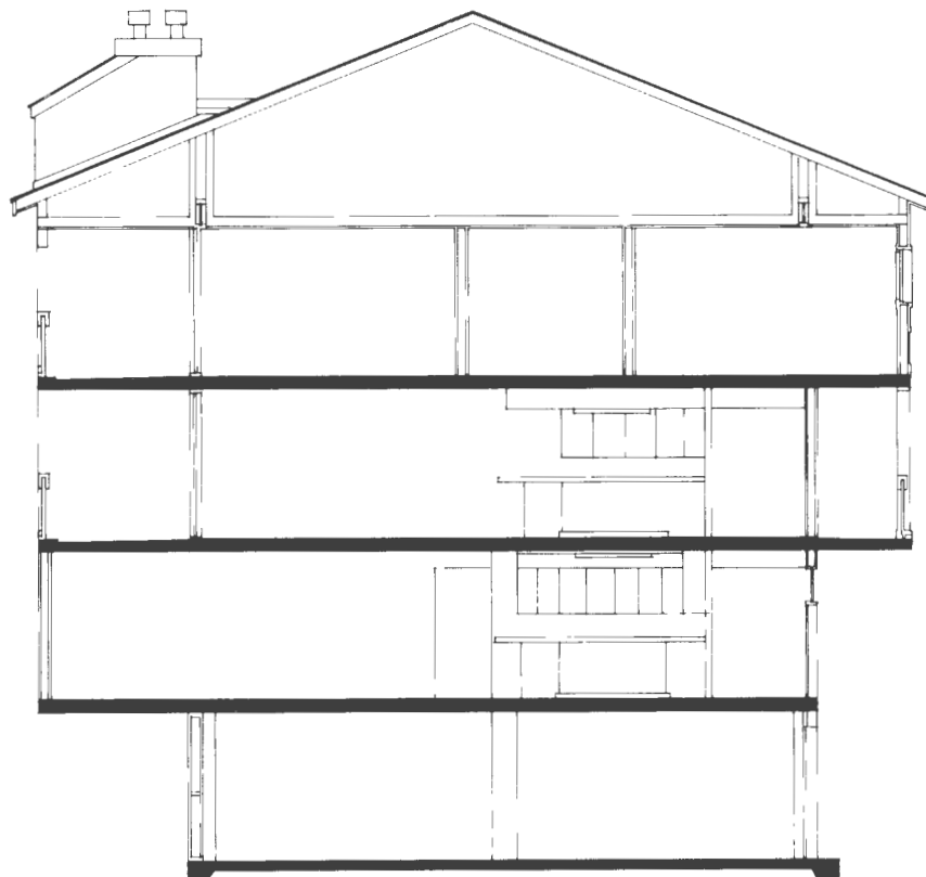
SECTION
