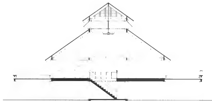
Figure 3.42 section
