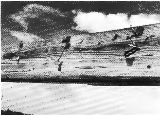
Figure 4.26. Toe Nailing Provides Limited Pull-Out Resistance
