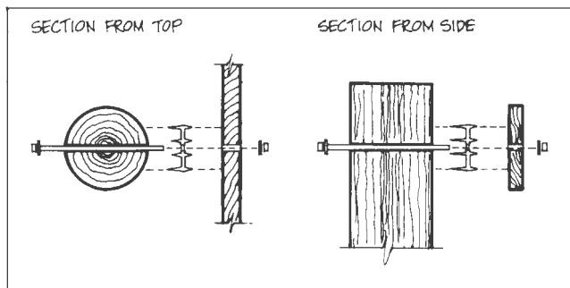
Figure 4.34. Spiked Grid
