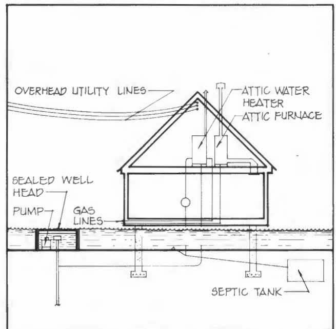
Figure 4.50. Locating Utilities
