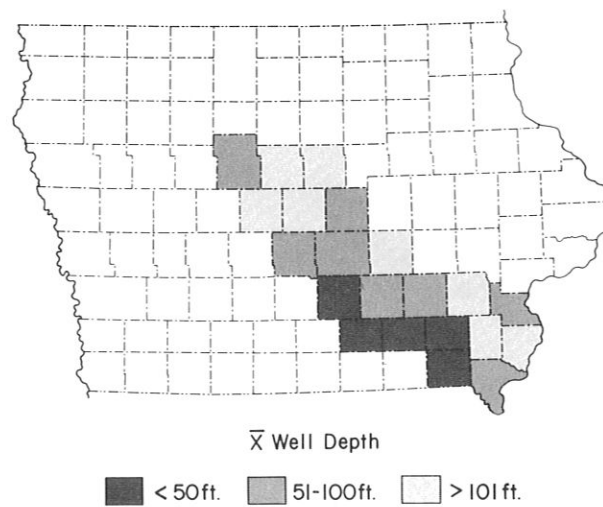
Figure 11. Mean well depth for all wells in a county.
