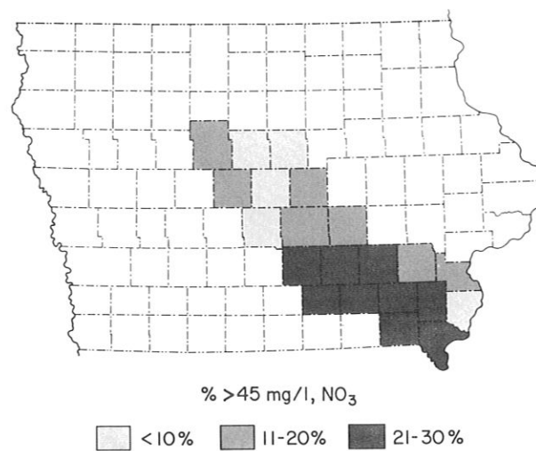
Figure 10. Percent of all analyses exceeding the nitrate MCL (45 mg/l NO 3 ).
